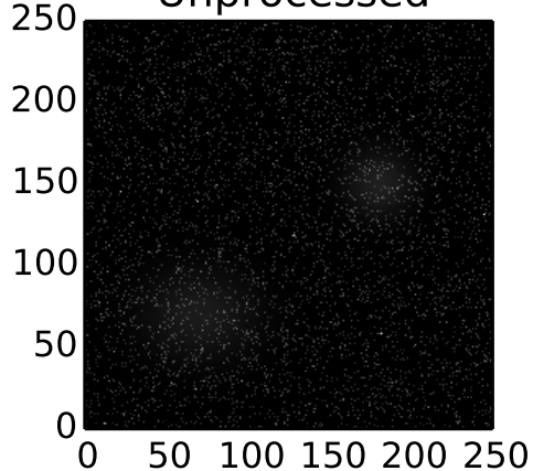
Unprocessed
