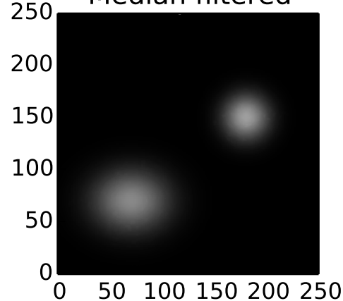
Median filtered
