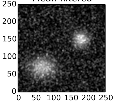
Mean filtered
